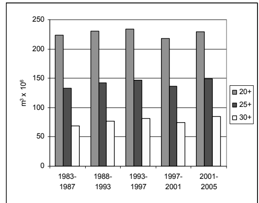
Figure 3. The volume of spruce trees (millions of m 3 ) in the area of Sweden where the northern Chiffchaff breeds (see Figure 1). The area includes Norrbotten and Västerbotten, Jämtland, Härjedalen, Ångermanland, Medelpad and Hälsingland. Values are five-year averages, for trees with 20, 25 and 30 cm diameter or more, respectively, starting at the time of the main population decline of Chiffchaffs (see Figure 1). Source: Swedish National Forest Inventory.
